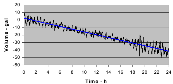
Figure 7. Level data obtained with the LRDP-24 system for Test 10.
