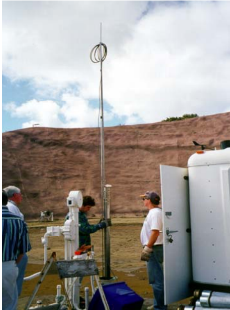
Figure 4. Photograph of the installation of the LRDP in the Point Loma tank.
