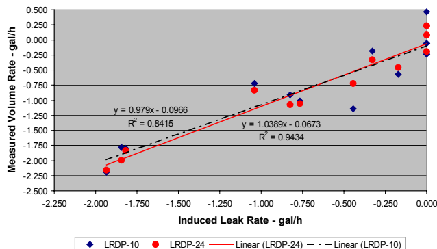
Figure 8. Least-squares lines fitted to the test results of the LRDP-10 and the LRDP-24.
