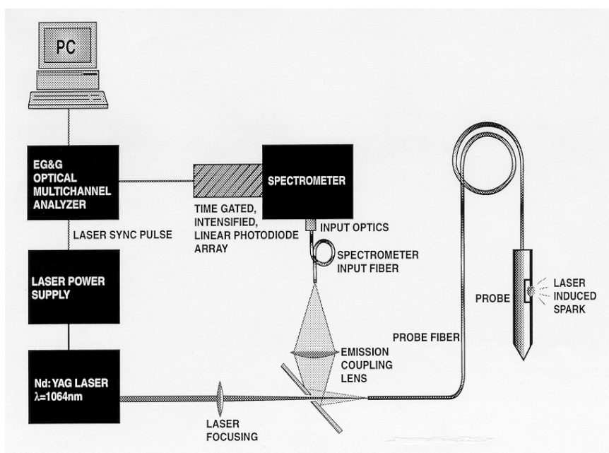
Figure 1. Schematic of Fiber Optic LIBS (FO-LIBS) System.
