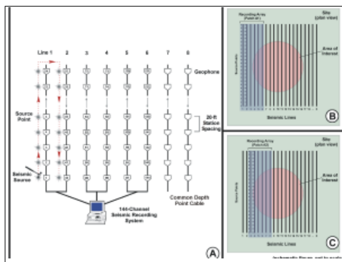
Figure 2. 3-D data acquisition schematic.
