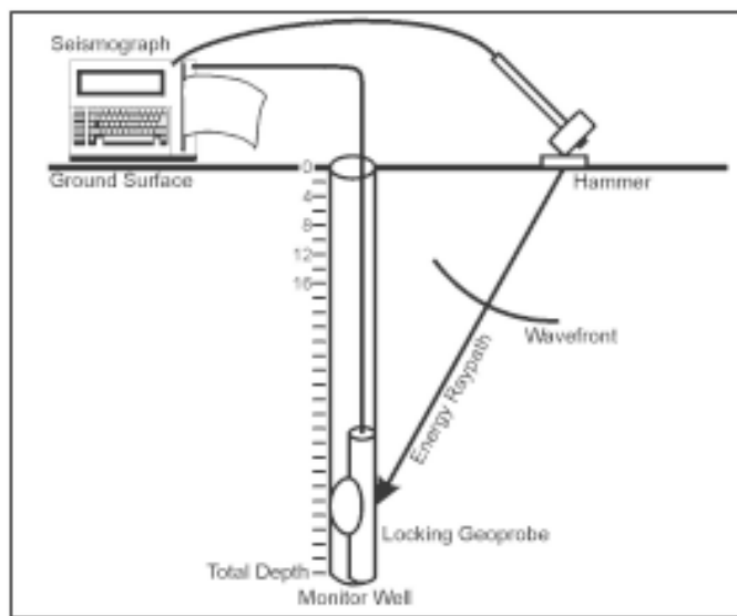
Figure 1. Vertical seismic profile schematic.
