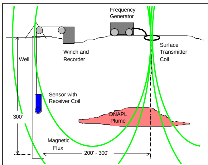
Figure 5. 3-D resistivity transmitter and receiver system.
