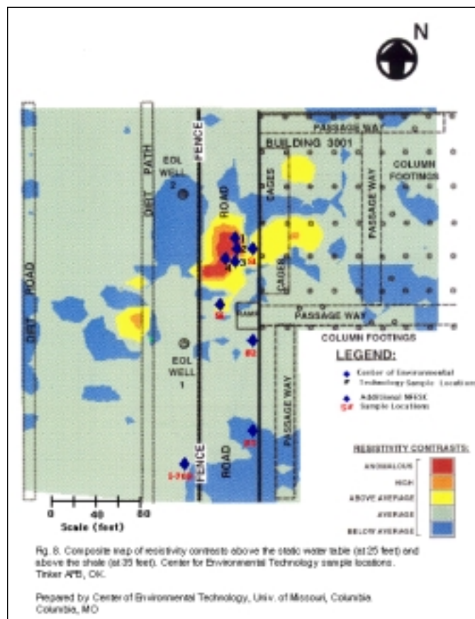
Figure 7. Composite map of resistivity contrasts.
