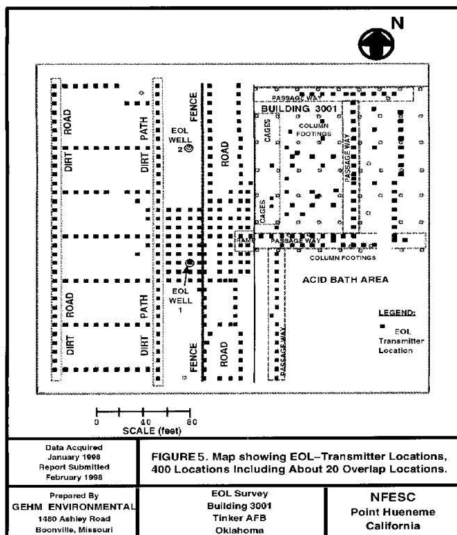
Figure 6. Transmitter locations - Tinker AFB.
