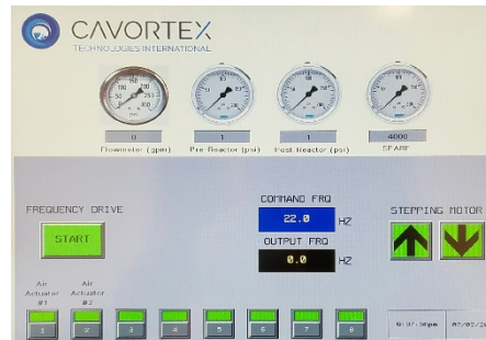
Cavitation Zone
